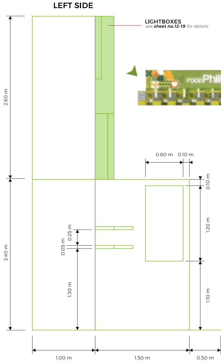
SIDE ELEVATION (EXHIBITOR)
