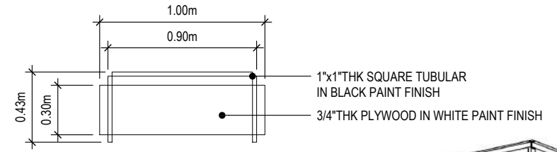
TOP VIEW
