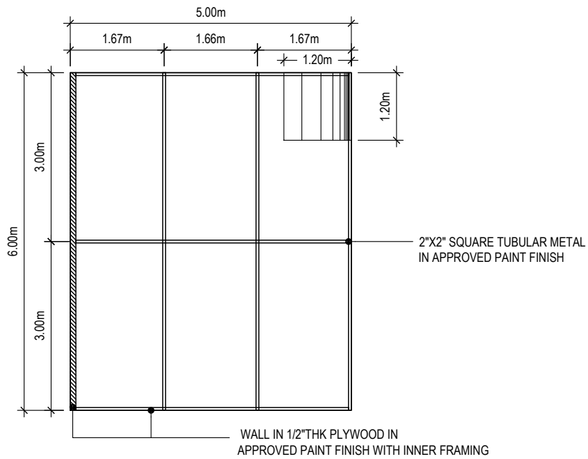
TOP VIEW
