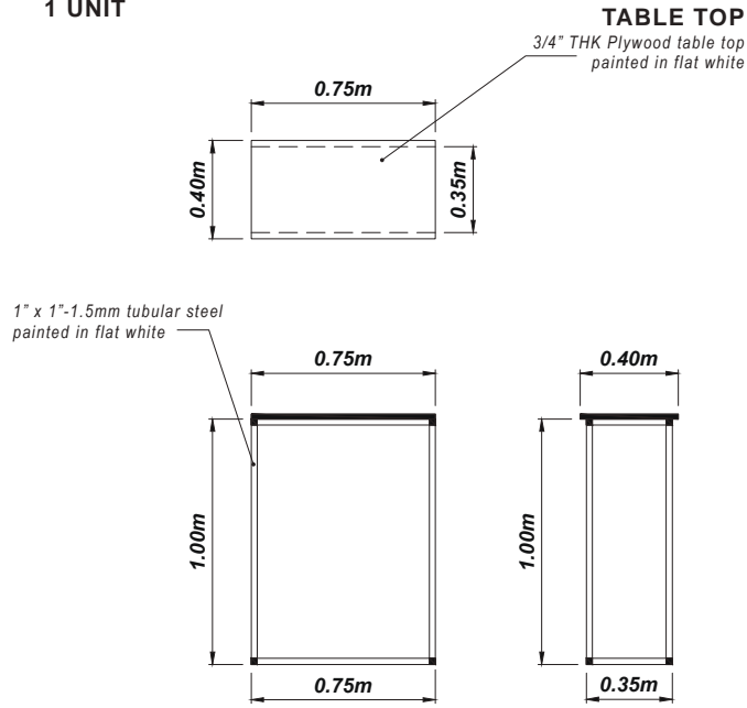
DISPLAY TABLE-01 1 UNIT
