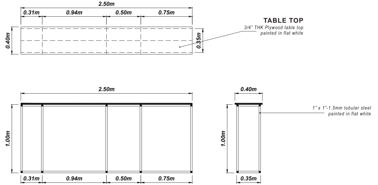
DISPLAY TABLE-02 1 UNIT
