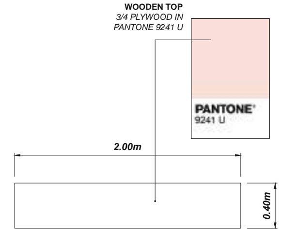
LOCKABLE CABINET 1 UNIT
