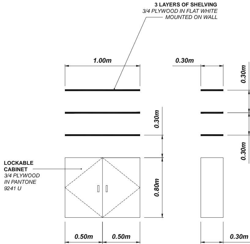
EXHIBITORS DISPLAY-01 38 SETS
