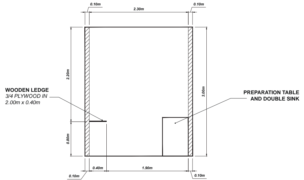
SECTION C-C
