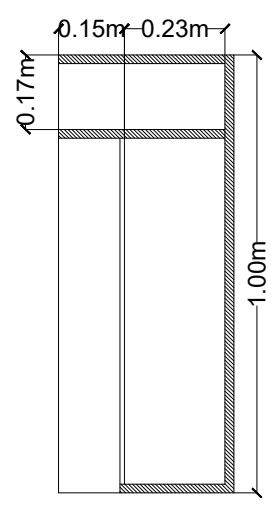
SECTION B
