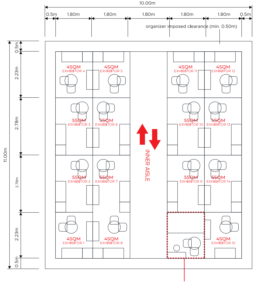
CITEM AREA (1.80m x 2.23m) see sheet no.08 for details
