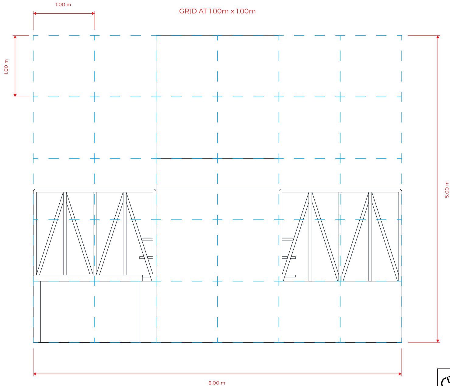
GRID FRONT LAYOUT PLAN
